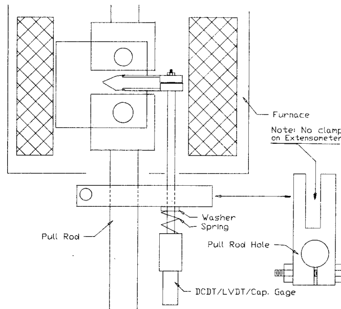
FIG. A1.5 Schematic of an Overall Test Set-Up Showing the Clip Gage as Attached to the Specimen
