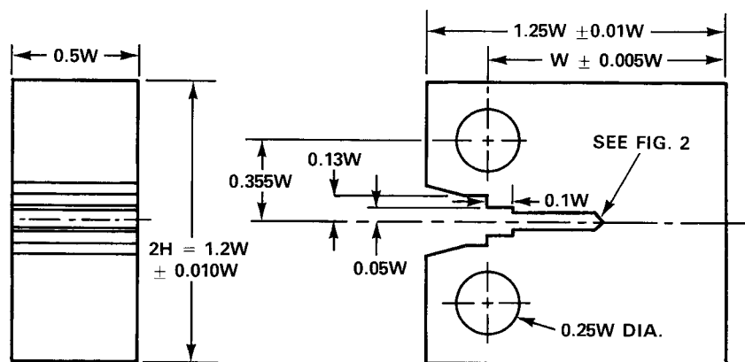
COMPACT TEST SPECIMEN FOR PIN OF 0.24W (+0.000W/−0.005W) DIAMETER FIG. A1.1 Drawing of a Standard C(T) Specimen with the Machining Tolerances
