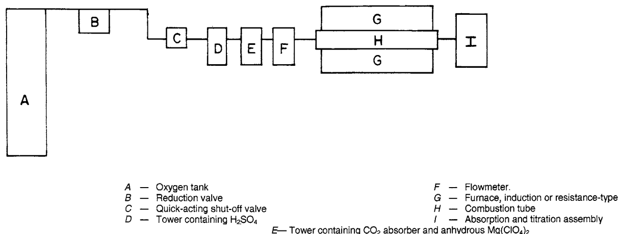
FIG. 1 Typical Arrangement for Determination of Sulfur by the Direct-Combustion Method
