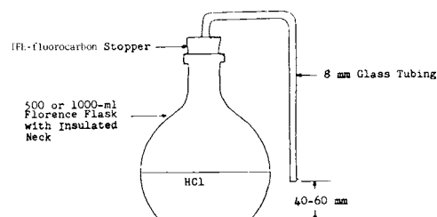
FIG. 2 HCl Gas Generator
