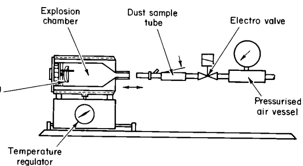
FIG. X2.2 Automated Version of the BAM Oven
