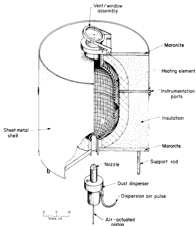
FIG. X4.2 Perspective Drawing of the Bureau of Mines 6.8-L Furnace
