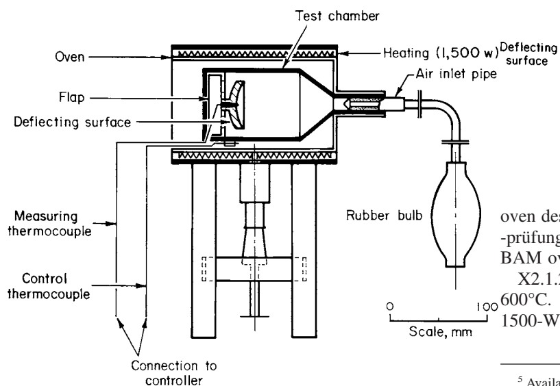
FIG. X2.1 Manually Operated Version of the BAM Oven
