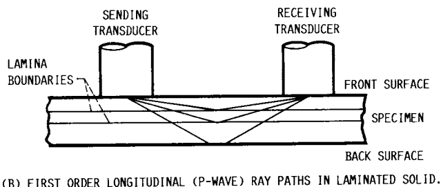
FIG. 3 Point Source-Receiver Ray Traces Illustrating the Development of AU Signals from Reflected Waves in a Monolithic and Laminated Solid
