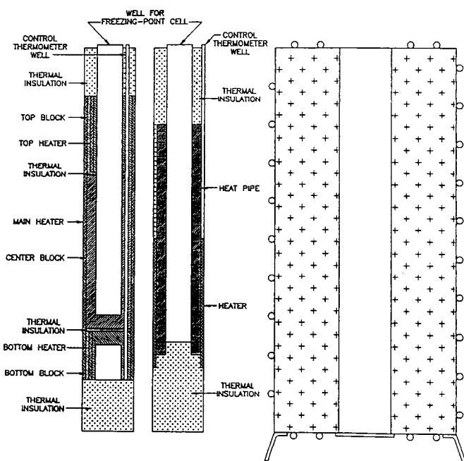
FIG. 1 Examples of Fixed-Point Cells
