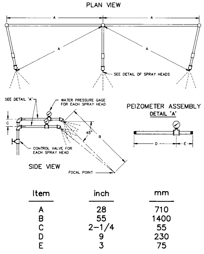
FIG. 8 Rain Test Spray-Head Piping
