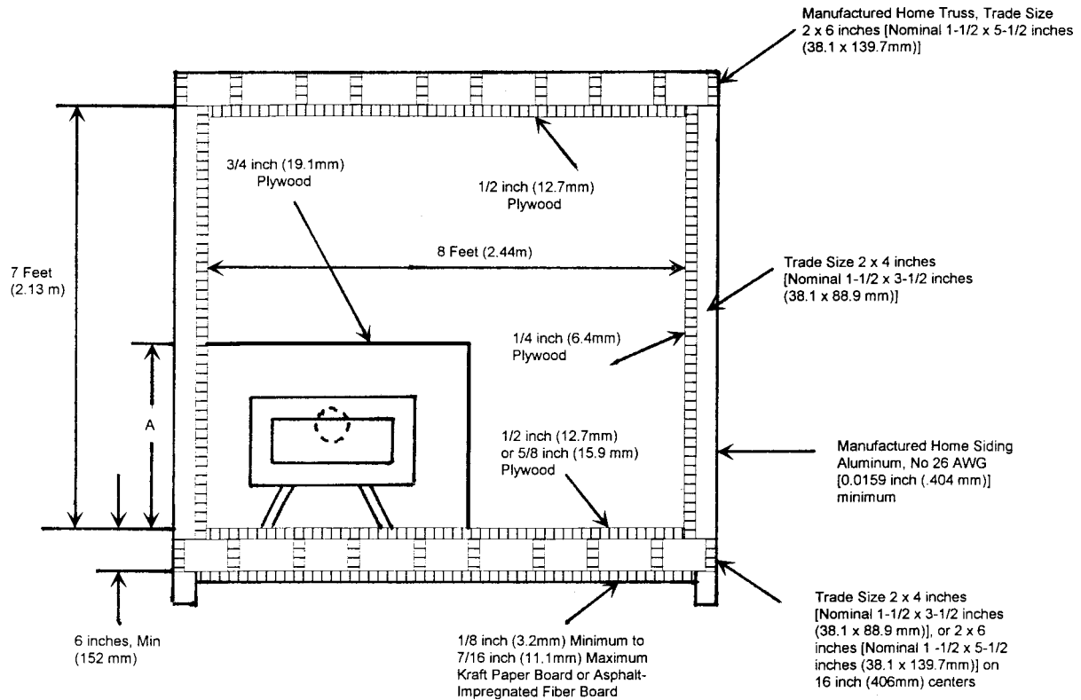
FIG. 1 Combined Conventional Home and Manufactured Home Test Structure (Shown with Optional Alcove Test Enclosure); Installation with a Direct Exhaust Venting System and Optional Alcove Enclosure
