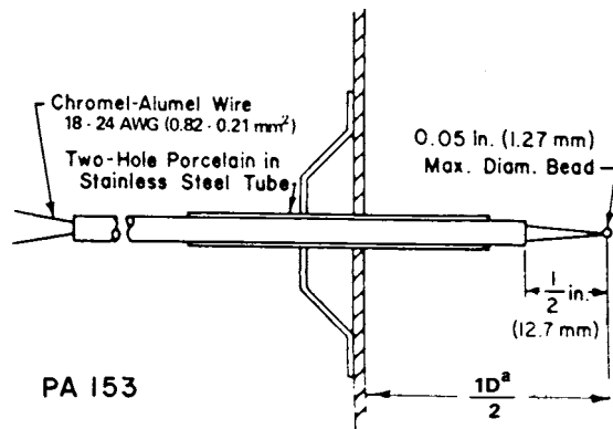
FIG. 4 Flue Gas Thermocouple and Support Bracket
