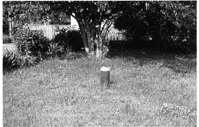
NOTE 1—Approximately 8-in. (203-mm) diameter. FIG. X1.10 Water Supply Well for Residential Property
