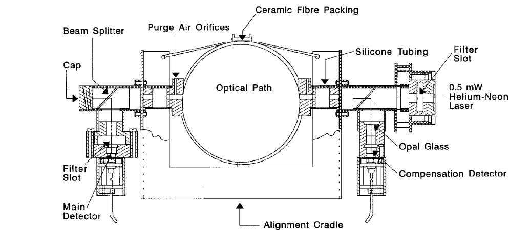
FIG. 11 Laser Extinction Beam
