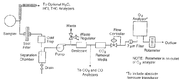
FIG. 9 Schematic of Gas Train
