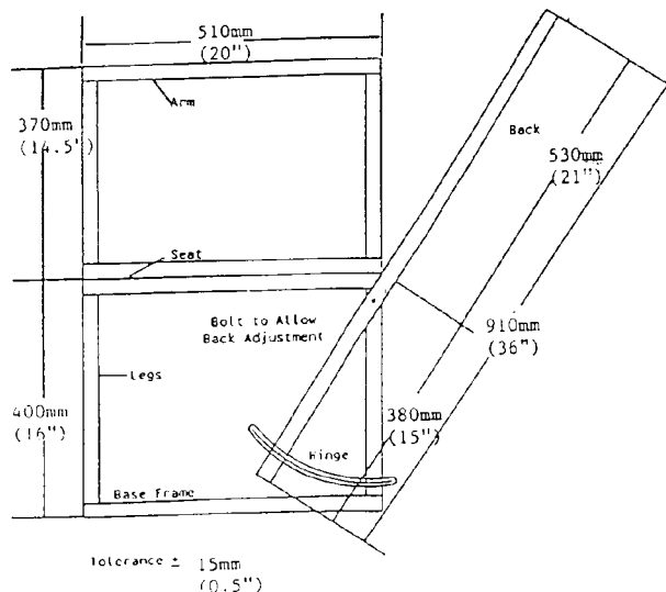
FIG. A1.2 Metal Test Frame (End View)
