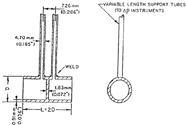
FIG. A3.1 Bidirectional Probe
