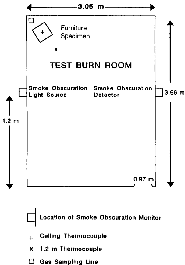
FIG. 2 Test Room Configuration for Option B for Items of Furniture Less Than 1 m Across
