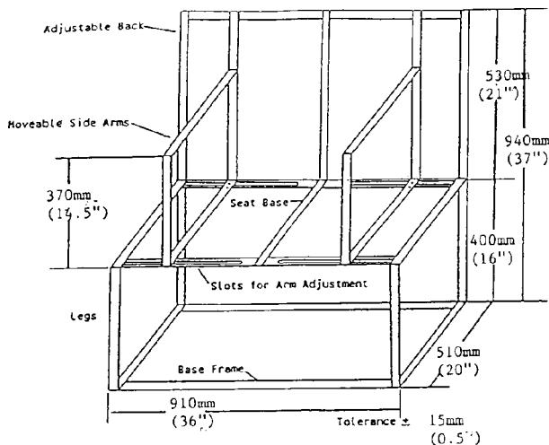
FIG. A1.1 Metal Test Frame
