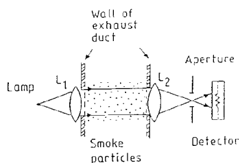
FIG. 10 Optical System, Using a White Light
