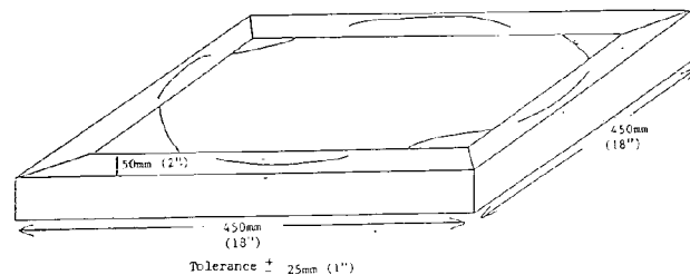
FIG. A1.3 Back View of Constructed Cushion
