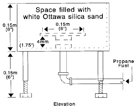
FIG. 12 Calibration Gas Burner
