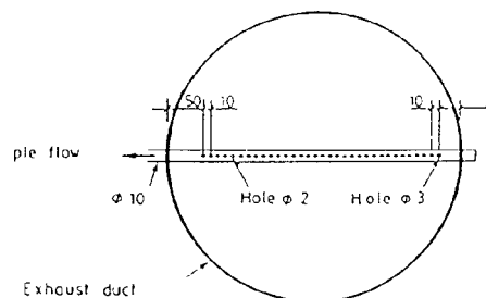
FIG. A3.2 Sampling Probe
