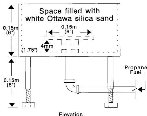
FIG. 12 Calibration Gas Burner
