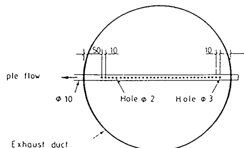
FIG. A3.2 Sampling Probe
