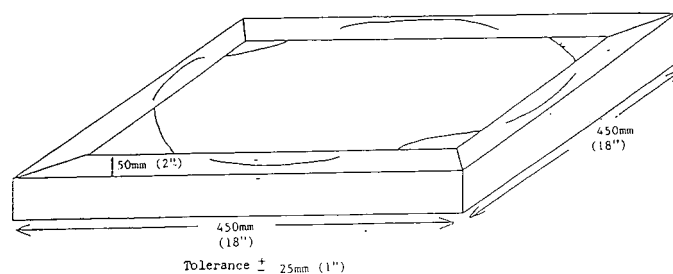
FIG. A1.3 Back View of Constructed Cushion
