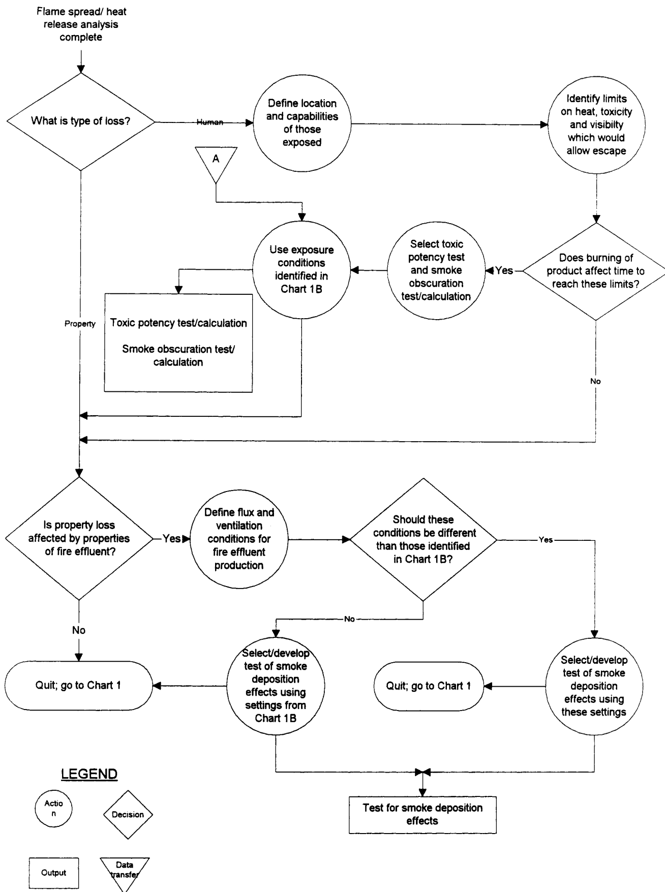
FIG. X4.4 Flow Chart 1C Fire Effluent Ref: 8.5.2.4 and 8.5.2.5
