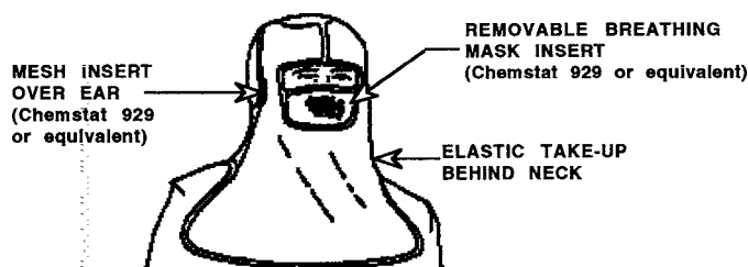
FIG. 3 Hood Detail
