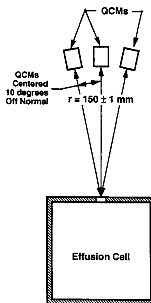
FIG. 3 QCMs—Effusion Cell Critical Dimensions
