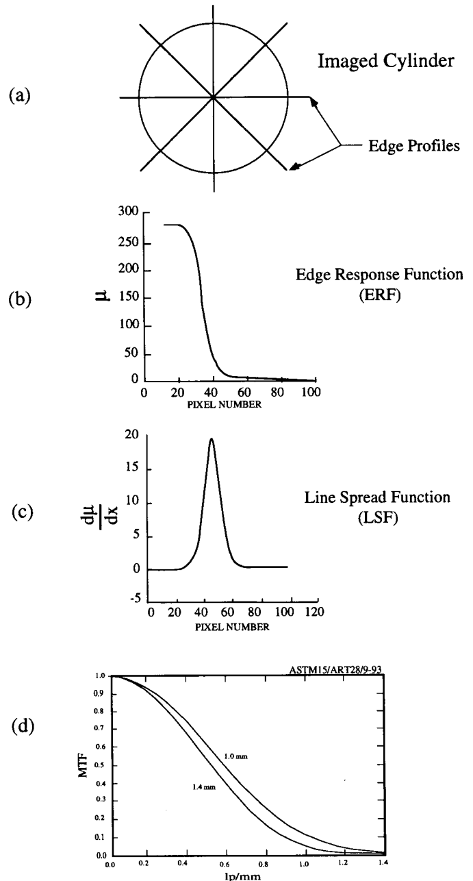
(a) An Illustration of One-Dimensional Profiles Through the Center of the Imaged Cylinder. (b) The Result of Aligning and Averaging Many Edge Profiles, the Edge-Response Function, ERF. (c) The System Line-Spread Function, LSF, Obtained by Differentiation of the ERF. (d) The System Modulation-Transfer Function, MTF, Obtained by Discrete Fourier Transformation of the LSF for Two Different Resolution Aperture Settings. The Smaller Aperture Setting Produces Slightly Better Modulation at Higher Frequencies.
