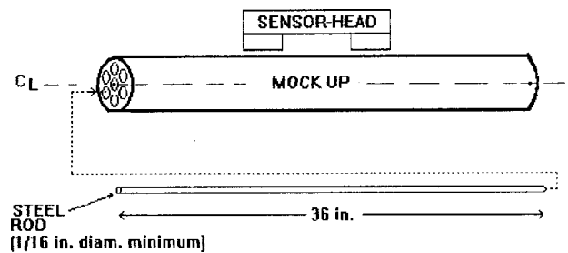
FIG. 5 Example of a Rod Reference Standard
