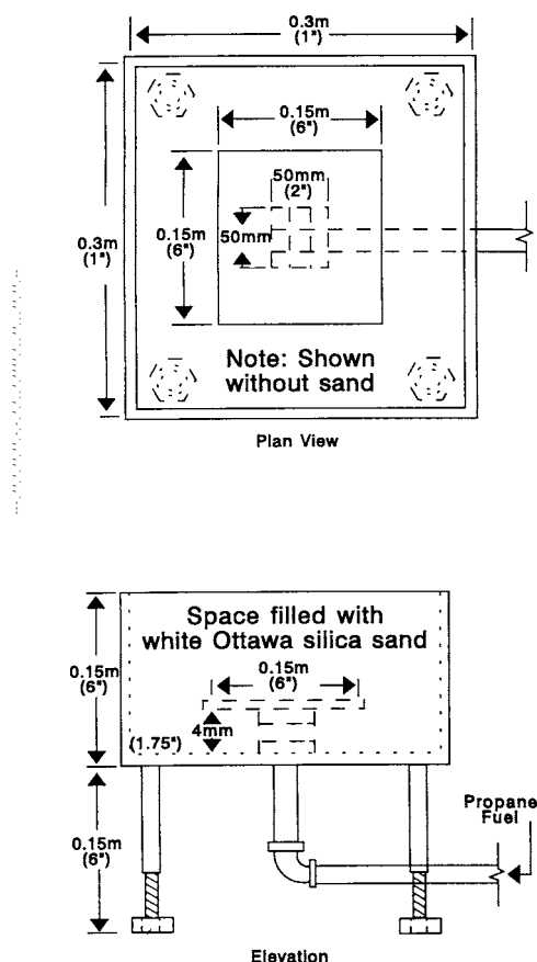
FIG. 12 Calibration Gas Burner
