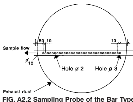
FIG. A2.2 Sampling Probe of the Bar Type
