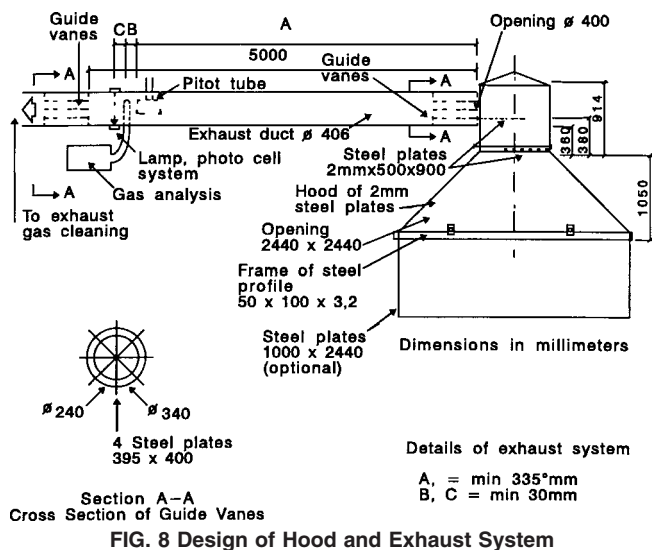
FIG. 8 Design of Hood and Exhaust System
