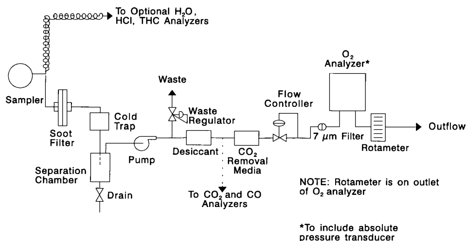
FIG. 9 Schematic of Gas Train
