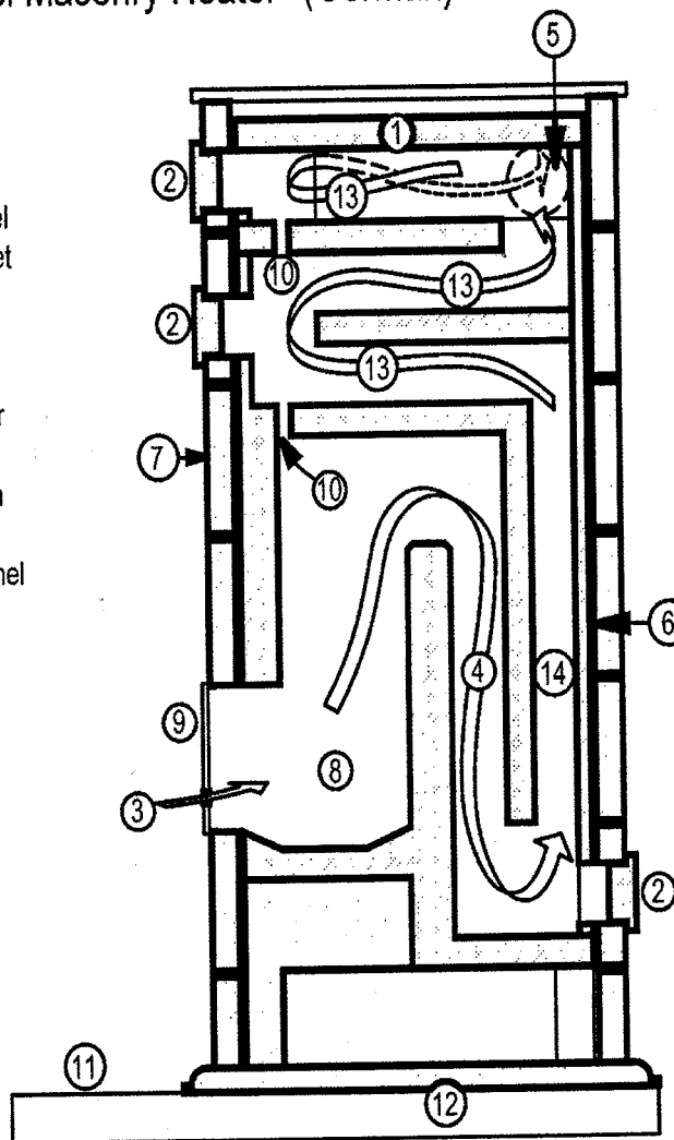
FIG. 3 Combination Vertical and Horizontal Channel Masonry Heater (German)
