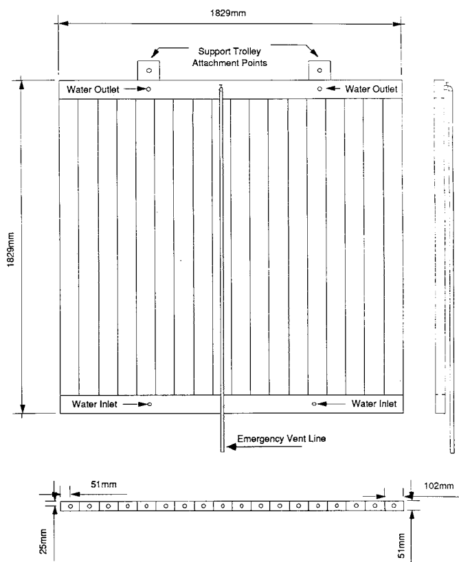
FIG. 4 Radiation Shield
