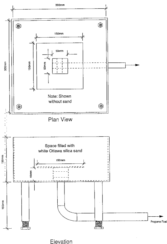
FIG. 9 Sand Burner
