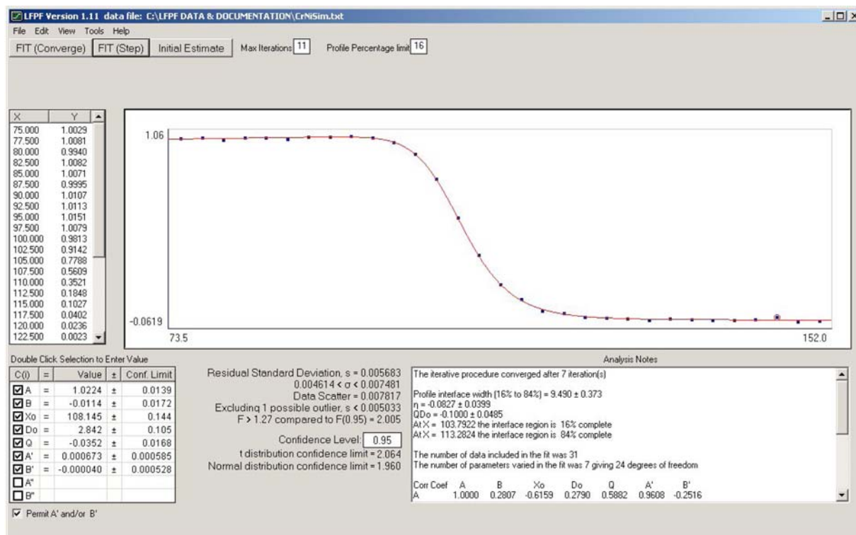
NOTE 1—The X-axis is sputtering time and the Y-axis is the normalized Cr Auger signal. FIG. X1.1 Results of a Least-Squares Analysis of Cr Disappearance in a Simulated Cr-Ni Interface
