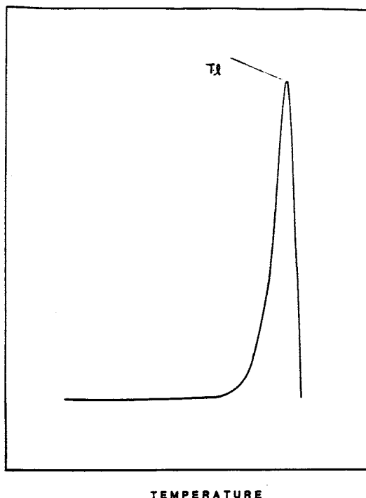
FIG. 2 Loss Modulus
