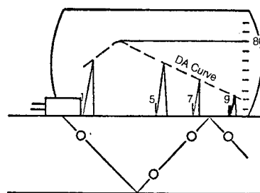
FIG. A2.5 Distance Amplitude
