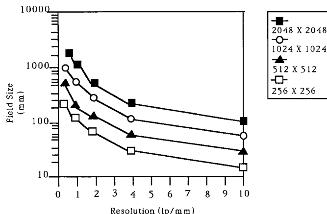
FIG. 2 Effect of Resolution on Field Size for Several Pixel Matrix Sizes
