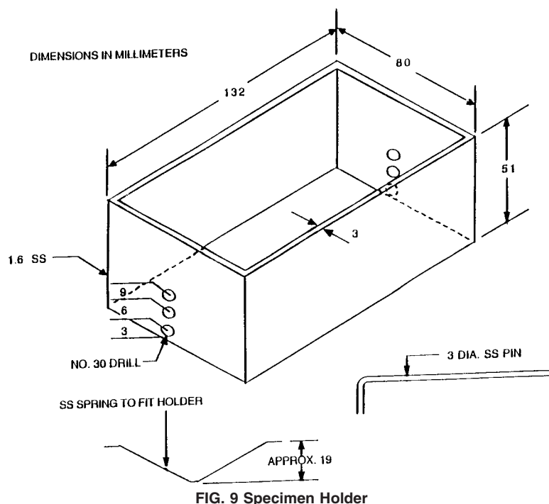
FIG. 9 Specimen Holder
