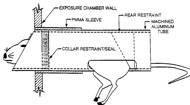
ANIMAL RESTRAINER
