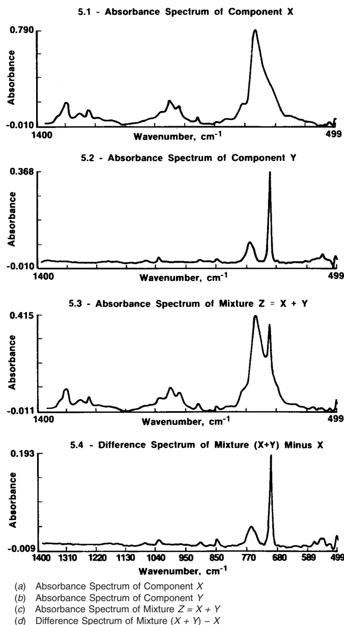
FIG. 5 An Example of Difference Spectroscopy
