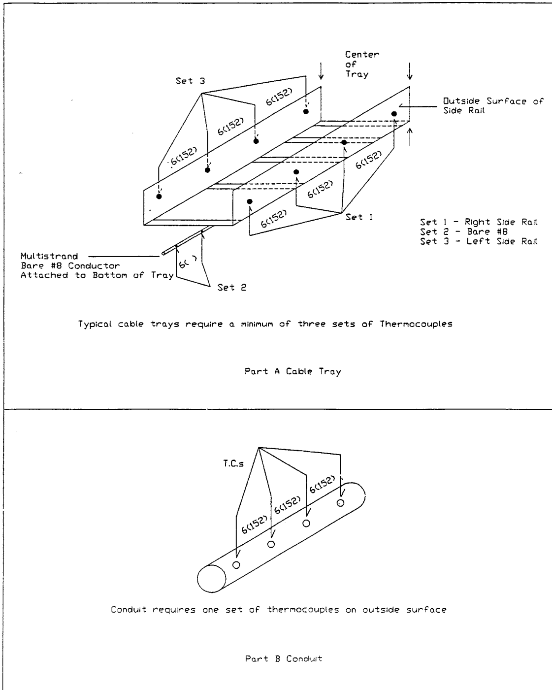
FIG. 7 Specimen Thermocouples
