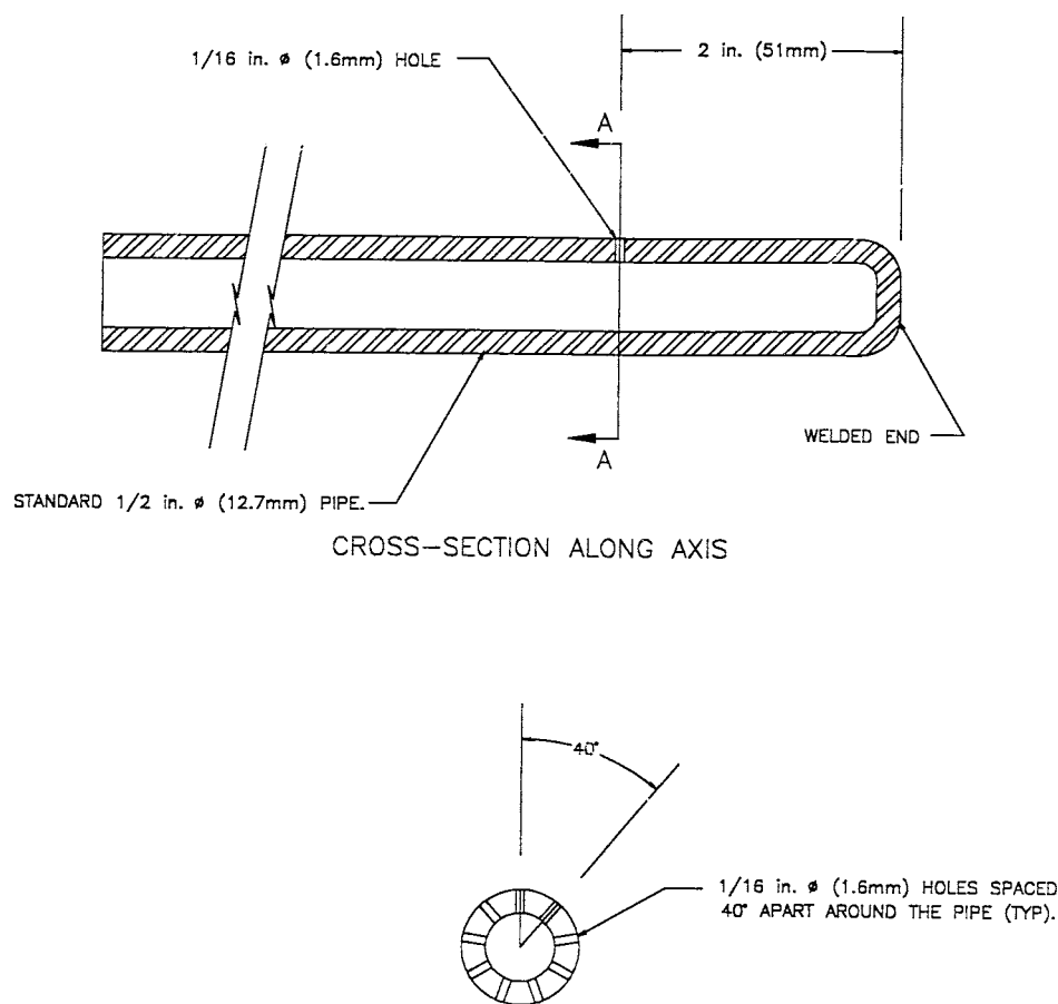
SECTION A-A FIG. 2 Furnace Pressure Probe 2
