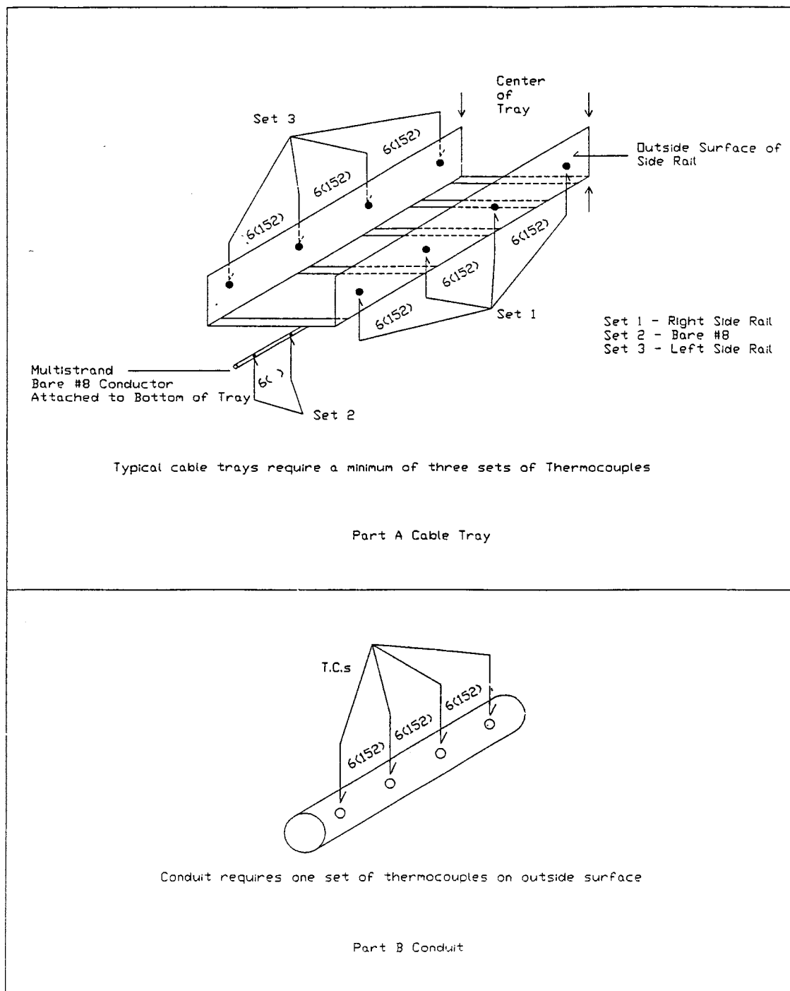
FIG. 7 Specimen Thermocouples
