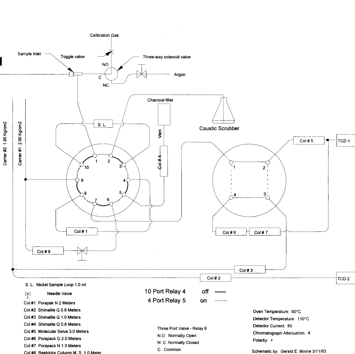
FIG. 1 Chlorine Impurity Analysis System Flow Diagram
