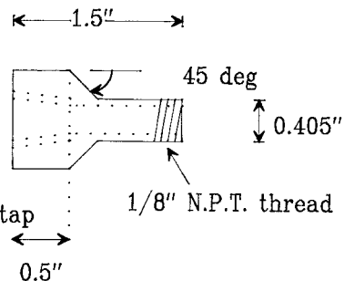
FIG. 1(a) Pipe Adapter
