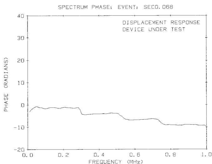
FIG. 7 Phase of the Frequency Response of the SUT Derived from the Data of Figs. 4 and 5
