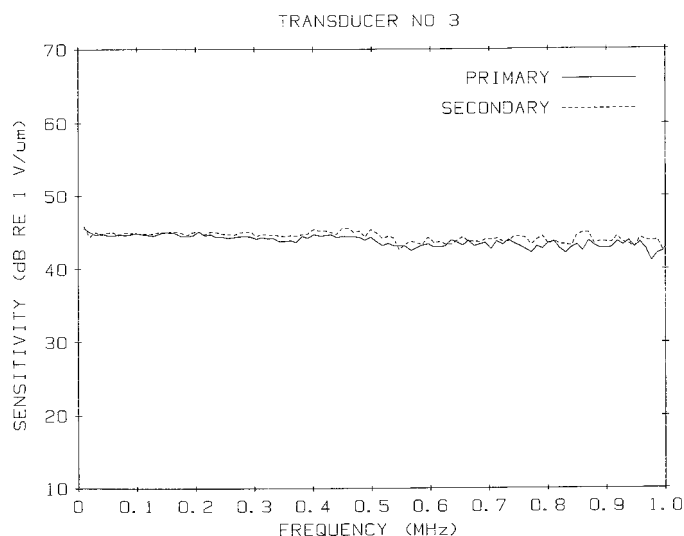
FIG. 9 Comparison of Primary and Secondary Calibration Results for an NIST Conical Transducer, Having an Aperture Diameter of 1.4 mm [0.055 in.]
