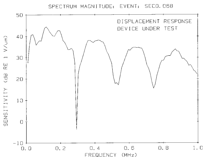
FIG. 6 Magnitude of the Frequency Response of the SUT Derived from the Data of Figs. 4 and 5
