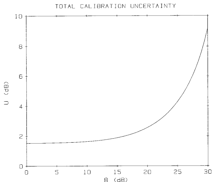
FIG. 8 Estimated Uncertainty, U , of the Calibration Frequency Response Data —Let M be the Largest Value of w_m over the Range 100 kHz to 1 MHz; Then, for any w_m , B = M - w_m , and the Uncertainty of w_m is \pm U
