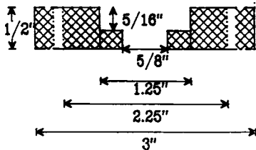
FIG. 7 Flange Detail
