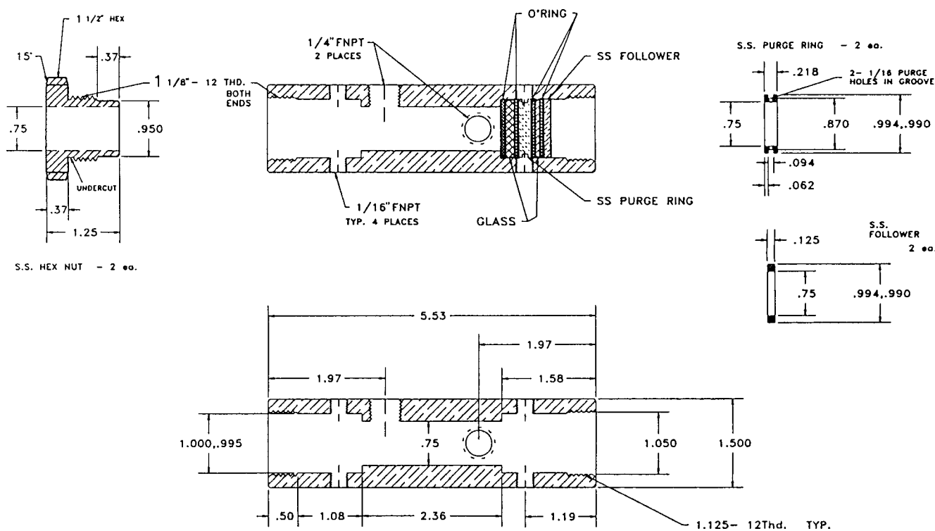
FIG. 9 Special Infrared Process Cell
