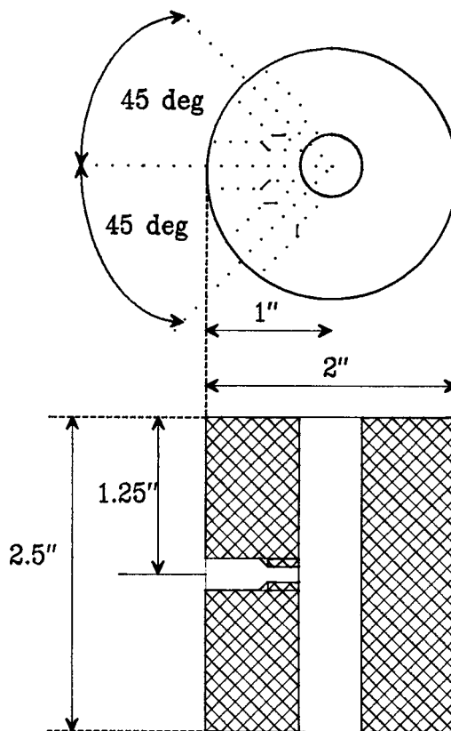
FIG. 4 Body Detail
