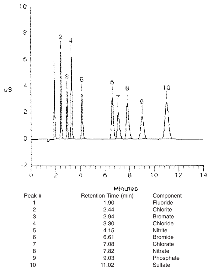
FIG. 1 Typical Chromatogram of Anions Eluting from a AS-12A Separator Column Using \text{Na}_2\text{CO}_3/\text{NaHCO}_3 Eluent
