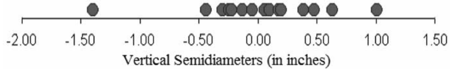
FIG. 2 Fifteen Residuals from the Semidiameters of Venus from Example 3 in 6.5.1
