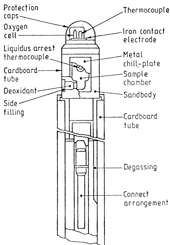
FIG. A1.5 Example of a Submergence Probe Assembly Showing the Sample Chamber
