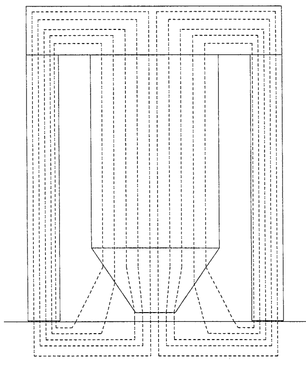
FIG. 10 Permanent Magnet Design for EMAT Pancake Coil in Fig. 9
