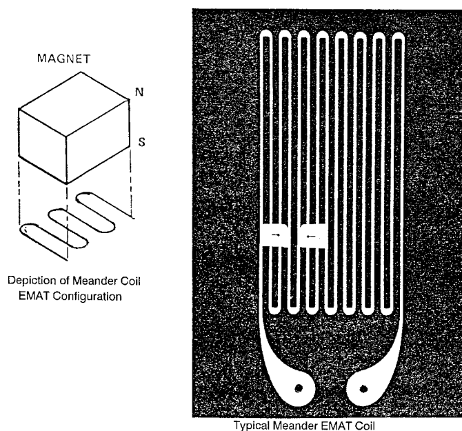
FIG. 4 Typical EMAT Meander Coil for Rayleigh Wave Generation
