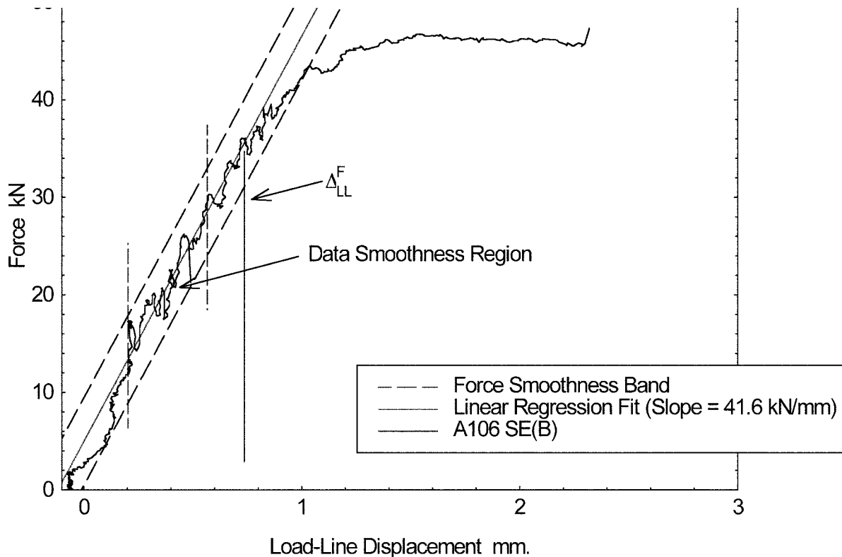
FIG. A14.7 Force Smoothness Verification Schematic
