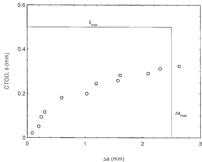
FIG. A10.1 Typical \delta - R Curve
