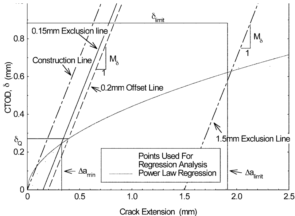
FIG. A11.1 Definition of Construction Lines for Data Qualification
