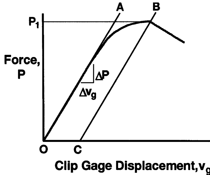
FIG. A4.3 Determination of Initial Compliance
