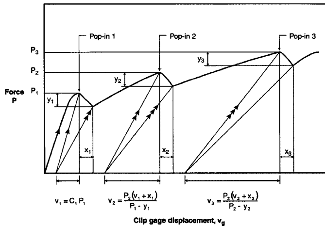
FIG. A4.1 Types of Force versus Clip Gage Displacement Records
