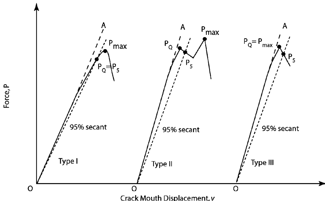
FIG. A5.1 Principle Types of Force-Displacement Records
