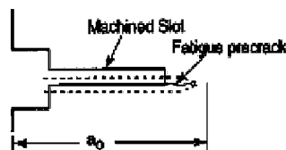
FIG. 7 Envelope of Fatigue Crack and Crack Starter Notches
