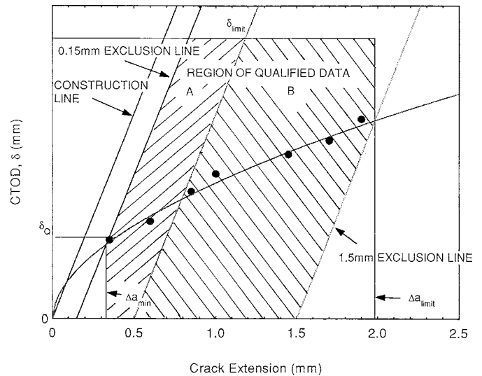
FIG. A11.2 Definition of Regions for Data Qualification
