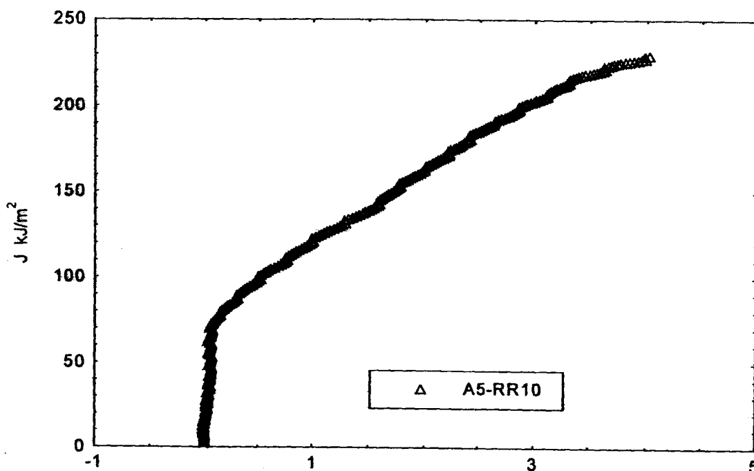
FIG. A15.5 The Resulting J - R Curve for this Specimen
