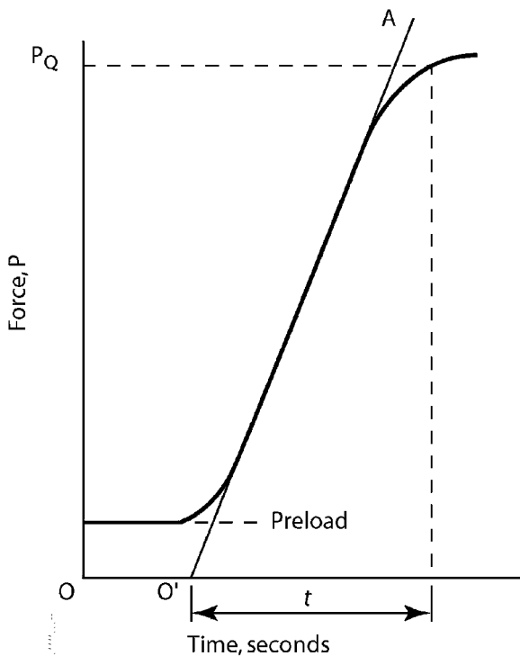
FIG. A13.2 Determination of Test Time from Force versus Time Record
