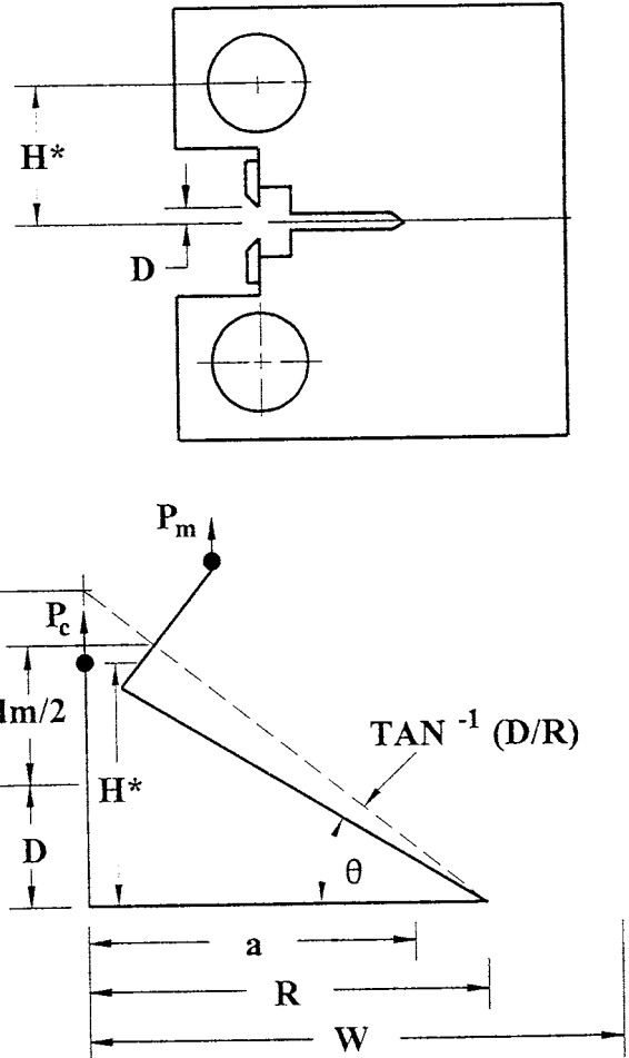
FIG. A2.3 Elastic Compliance Correction for Specimen Rotation
