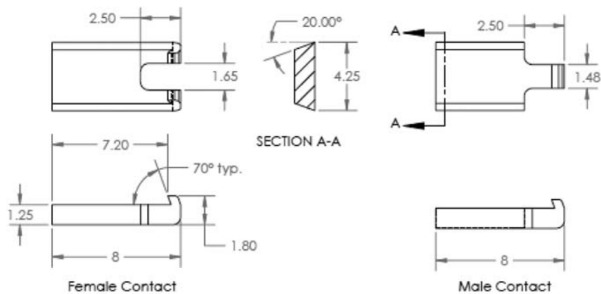
FIG. X2.2 Alternative crack opening displacement gage suitable for use with very narrow Notches.
