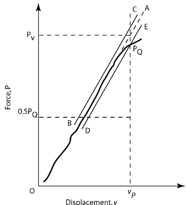
FIG. A13.1 Special Requirements for Analysis of Force versus Displacement Records (5 % Secant Line Not Shown)
