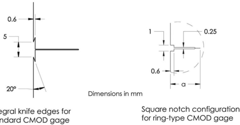
FIG. X2.1 Recommended notch configurations with integral features for mounting crack mouth opening displacement gages. These notch configurations are only recommended for a \geq 2\text{ mm} (0.079 in.)
