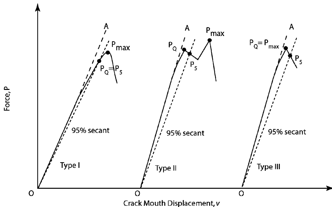
FIG. A5.1 Principal Types of Force-Displacement Records
