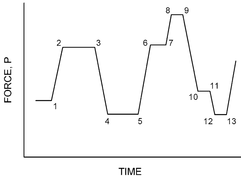
Example of Definitions Hold Times: 2-3, 4-5, 6-7, 8-9, 10-11, 12-13 Peaks: 2-3, 8-9 Valleys: 4-5, 12-13 Reversals: 3, 5, 9, 13
