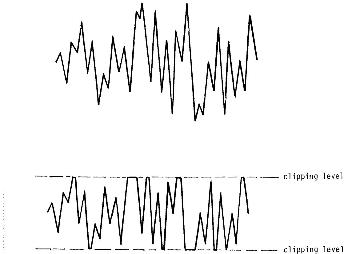
FIG. 3 Clipping of Fatigue Spectrum Loading
