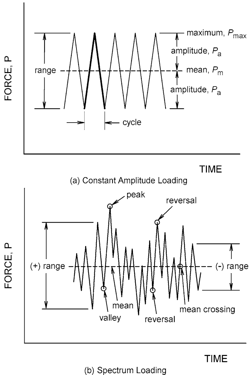
FIG. 4 Fatigue Loading Basic Terms
