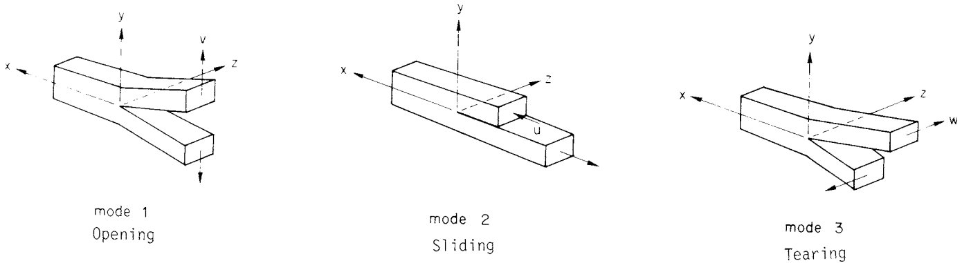
NOTE—See definition of mode. FIG. 8 Basic Modes of Crack (Surface) Displacements for Isotropic Materials
