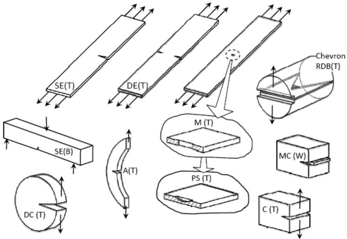
FIG. A2.2 Examples of Designation Codes for Specimen Configuration and Applied Loading
