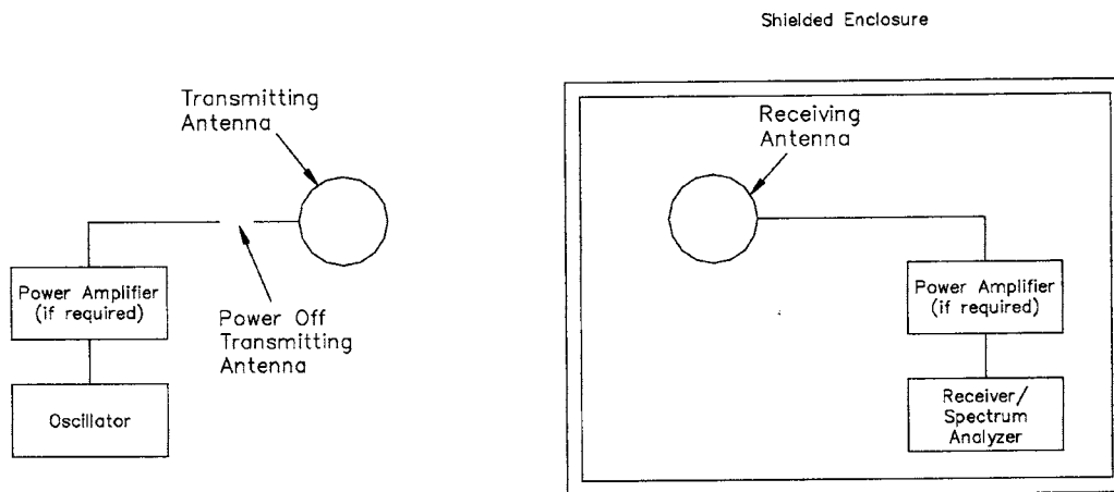
a. Magnetic Field Noise Measurement
