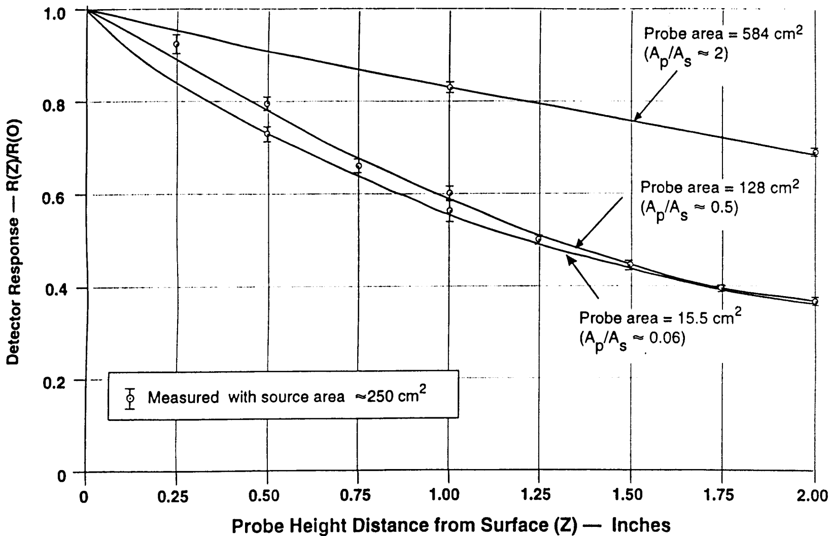
FIG. X4.3 Comparison of Detector Response for Various Probe Areas to a Large Area Source
