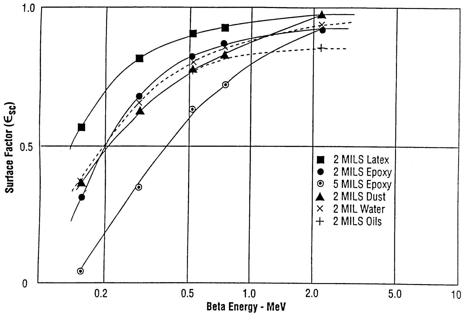
FIG. X5.2 Beta Measurement Surface Factor ( \epsilon_{sc} )
