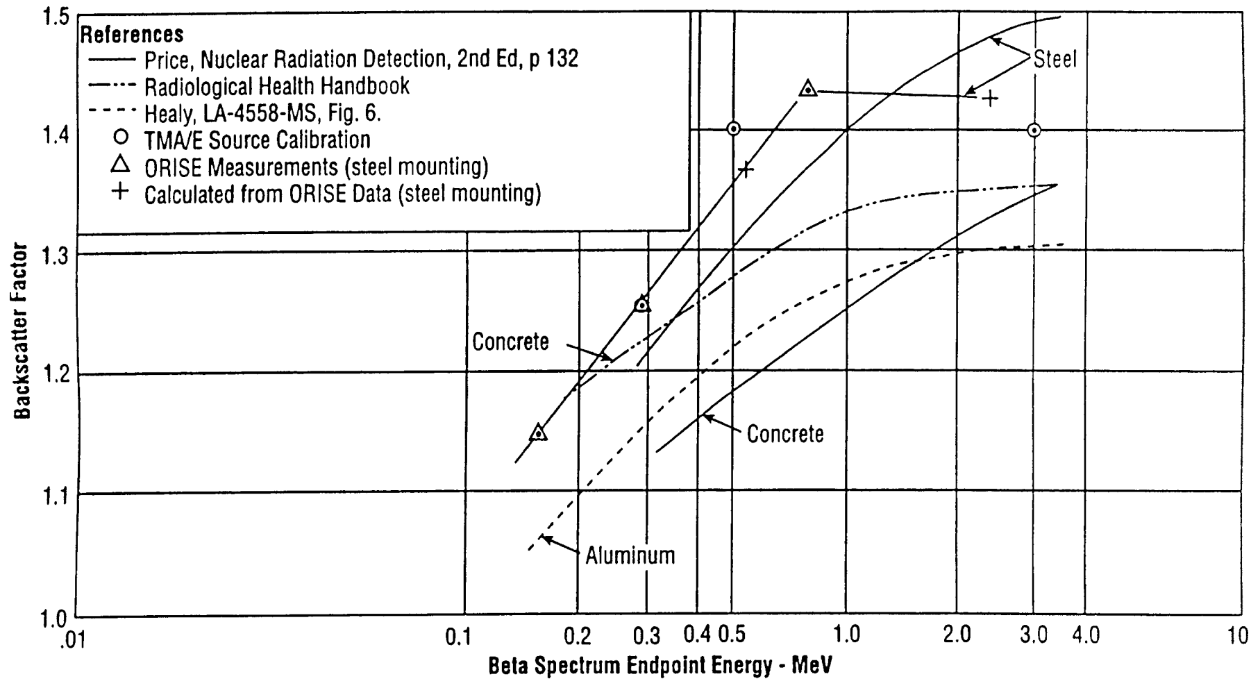
FIG. X8.1 Beta Backscatter from Various Surfaces
