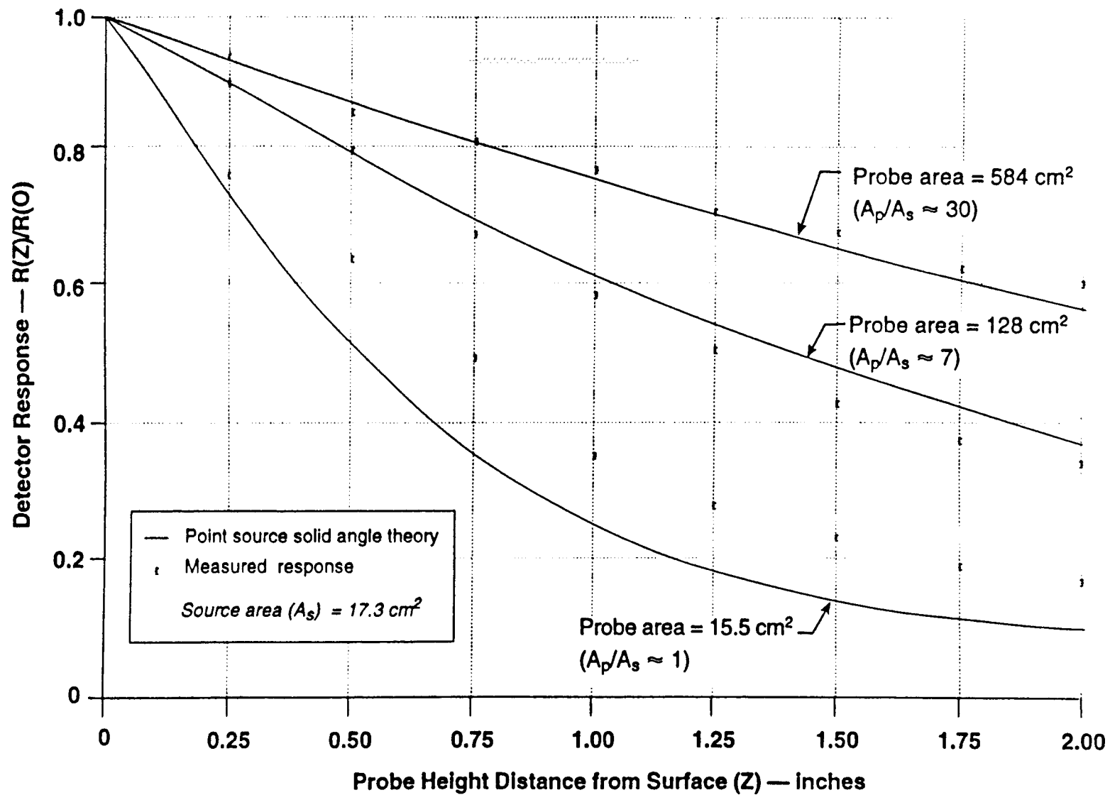
FIG. X4.2 Comparison of Detector Response to Point Source Theory for Various Probe Areas and a Small Area Source
