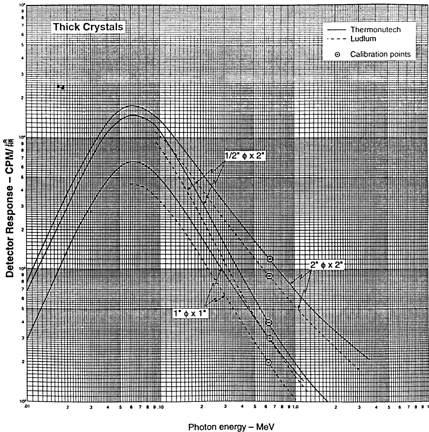
FIG. X7.1 Response vs Photon Energy for NaI Detectors
