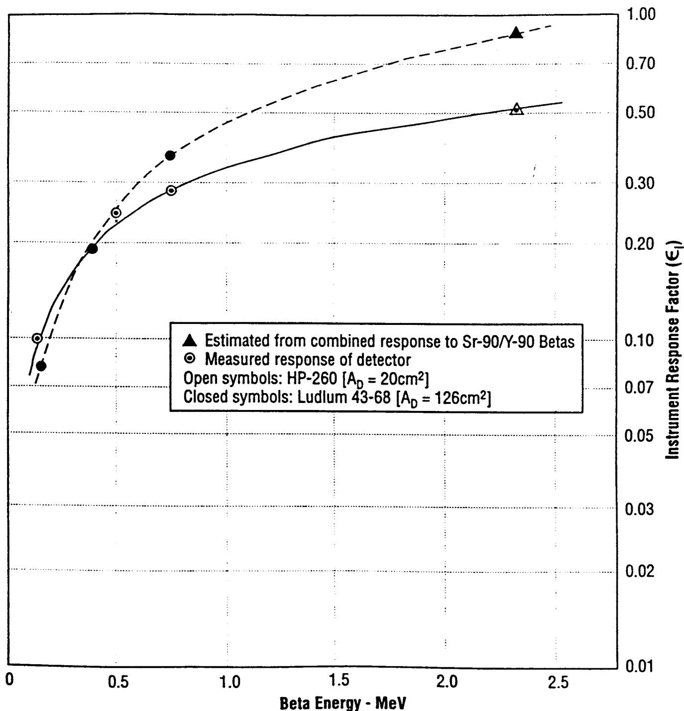
FIG. X6.1 Beta Instrument Response Factor ( \epsilon_I )
