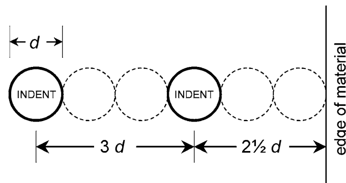
FIG. 3 Schematic of Minimum Indentation Spacing
