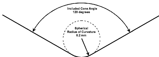
FIG. A3.1 Diagram of Cross-Sectional View of Spheroconical Diamond Indenter Tip
