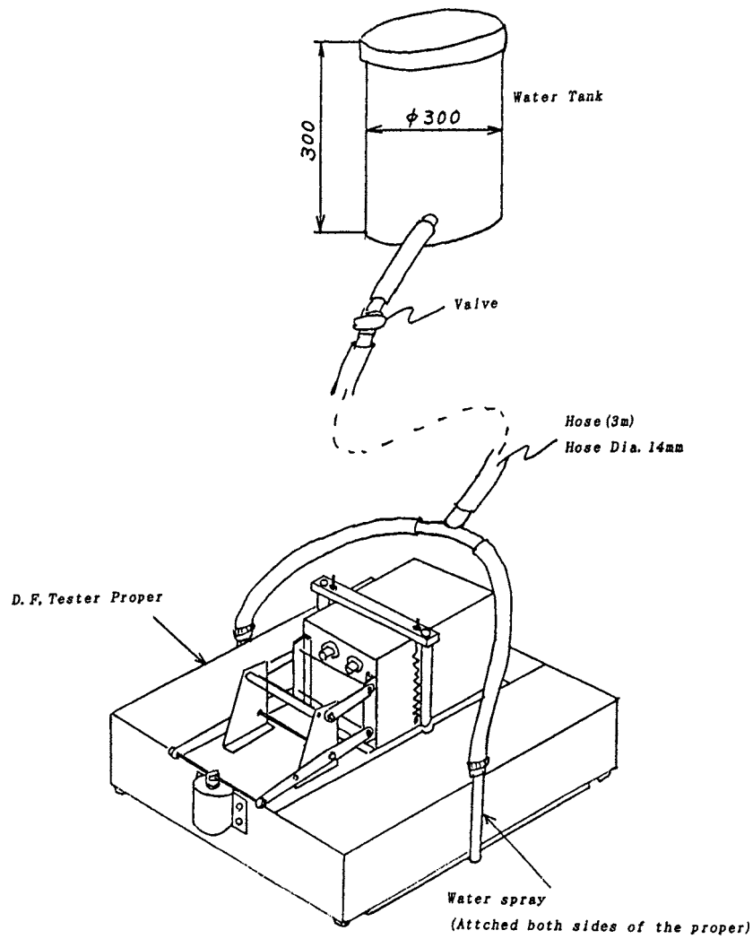
FIG. 2 The Watering Apparatus
