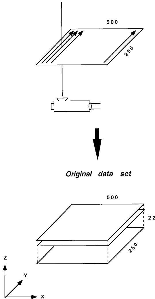
FIG. 5 Typical CST Imaging Scan Plan
