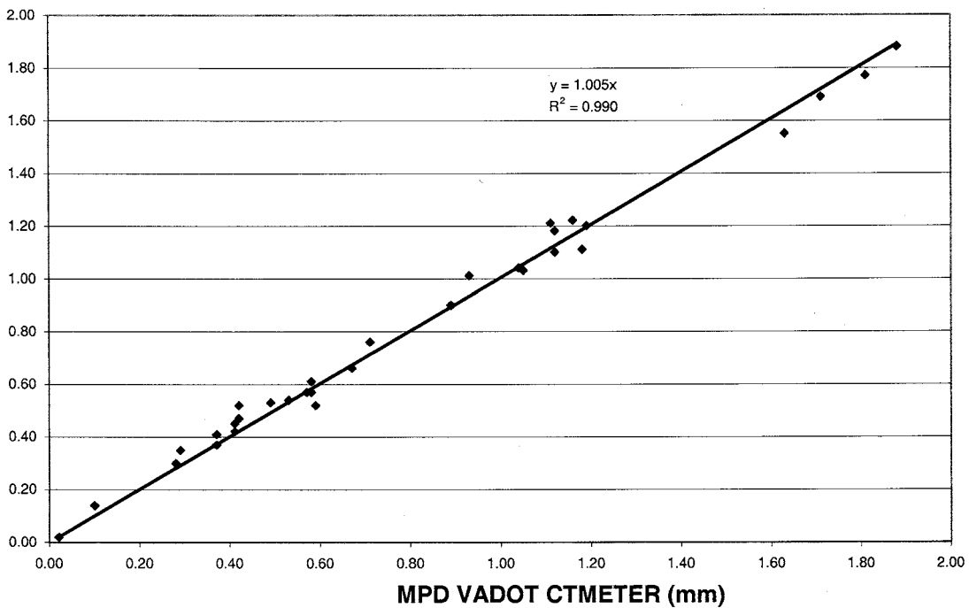
FIG. 2 MPD 2001 & 2002 Data for Two CTMeters
