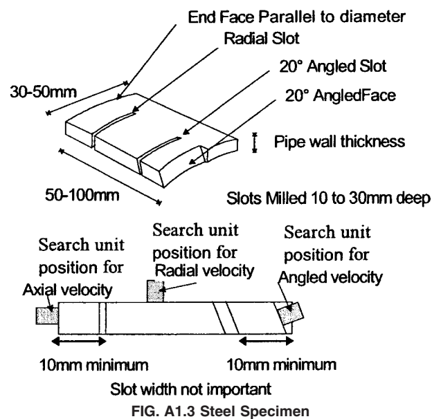
FIG. A1.3 Steel Specimen
