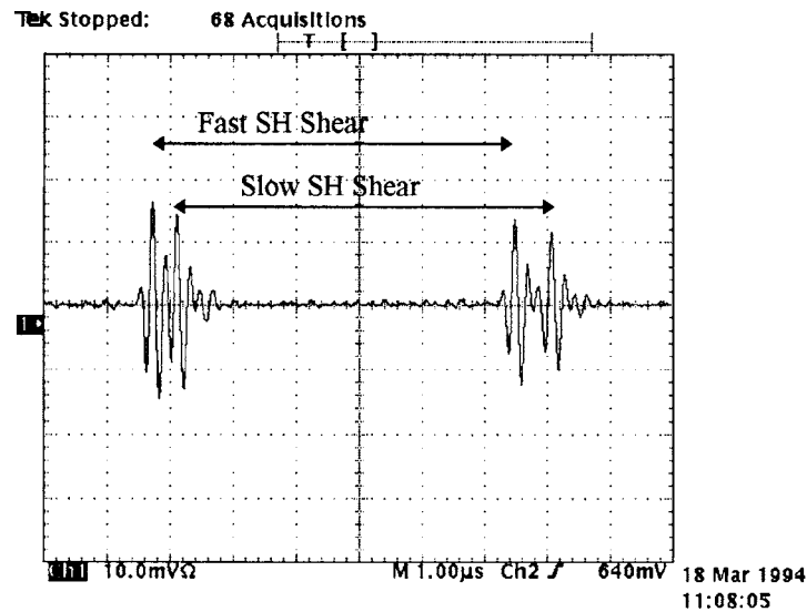
FIG. A1.2 Example of Time Interval Measured in Birefringent Material
