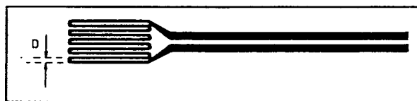
FIG. 2 Typical EMAT Meander Coil for Generation of Surface Waves
