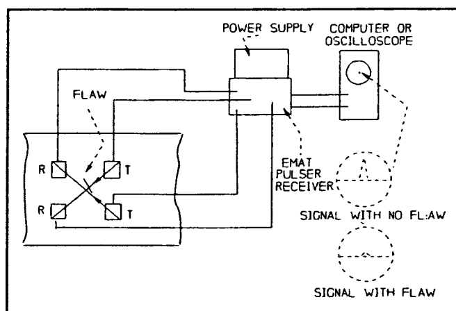
FIG. 3 Attenuation Technique
