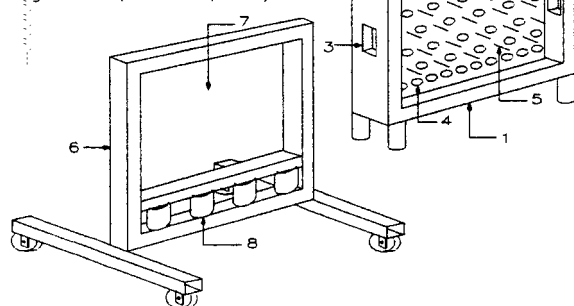
FIG. 1 Example of Vertical Furnace and Test Frame
