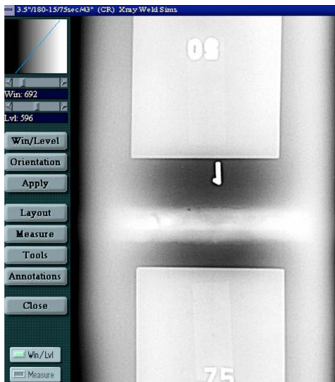
FIG. 27 Pipe Weld Features with Higher Win-Levels
