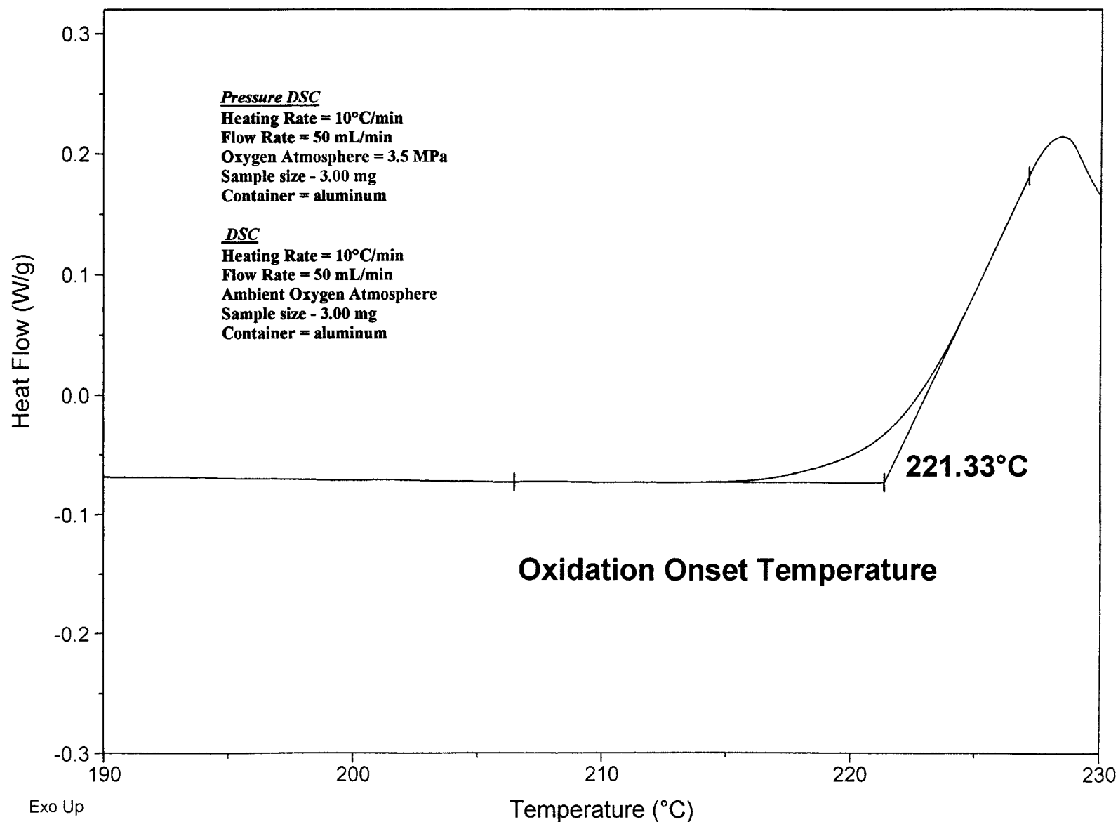
FIG. 1 DSC Oxidation Onset Temperature (OOT), Extrapolated Onset Temperature
